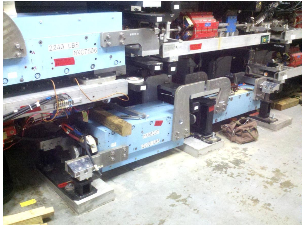
Hall D line Dipole Installation
