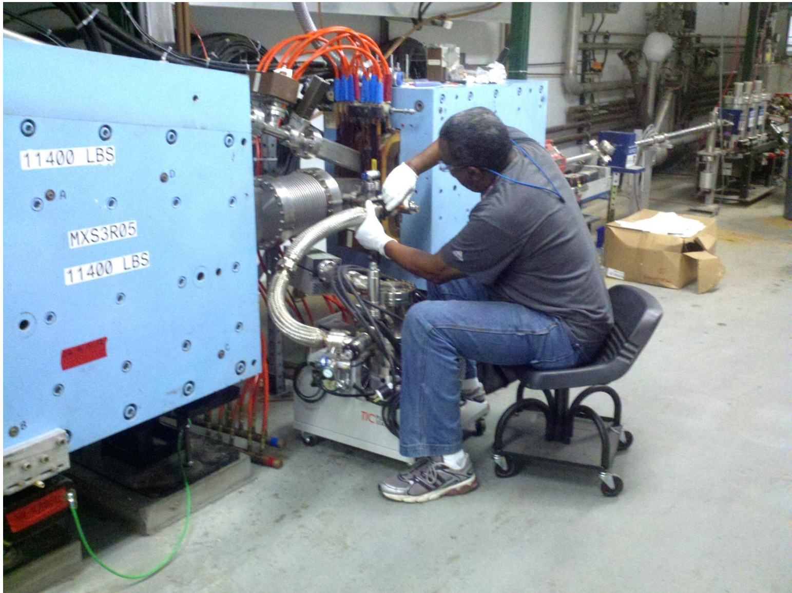
Completion of East Recombiner Vacuum Installation
